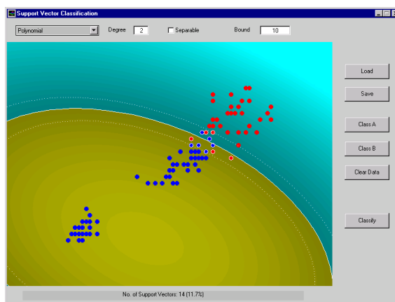
FIGURE 4.6: Separating Viginica with a polynomial SVM (degree 2, C = 10 )
