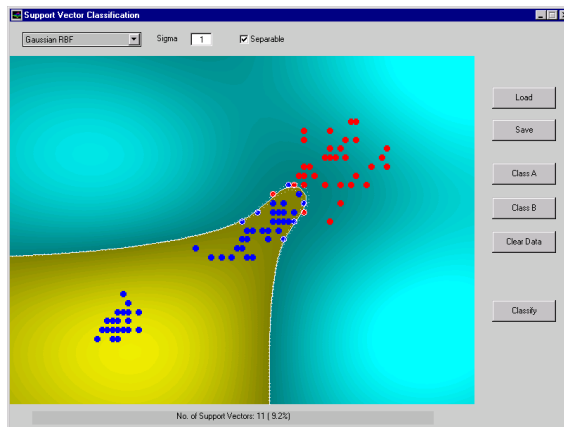
FIGURE 4.5: Separating Viginica with a Radial Basis Function SVM ( \sigma = 1.0 , C = \infty )
