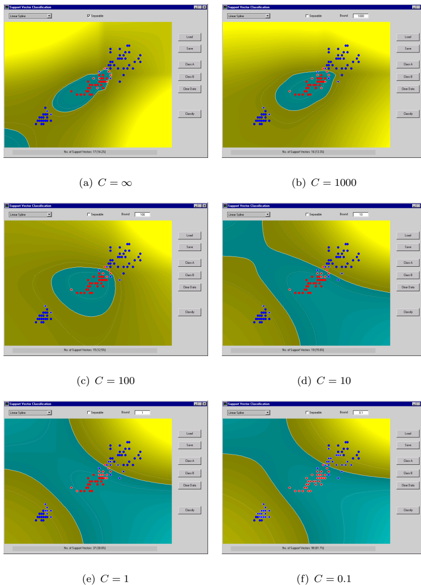
FIGURE 4.7: The effect of C on the separation of Versicolor with a linear spline SVM
