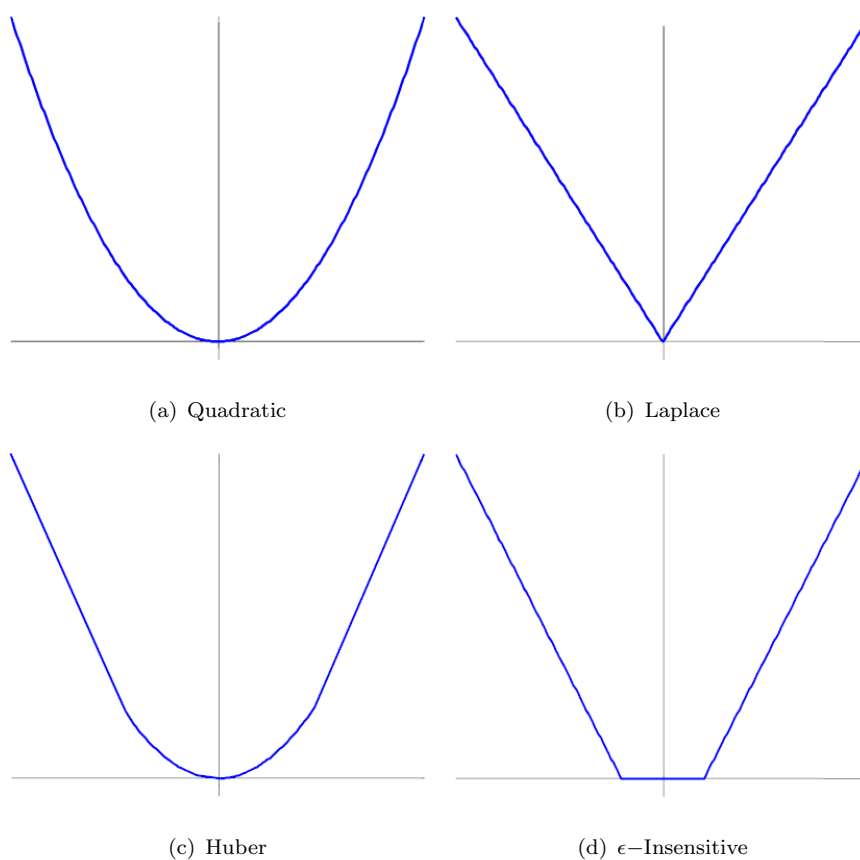
FIGURE 5.1: Loss Functions
