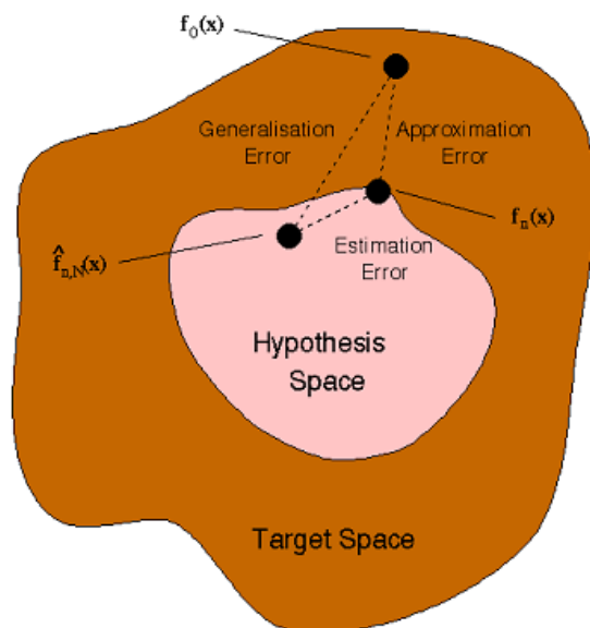
FIGURE 1.1: Modelling Errors
