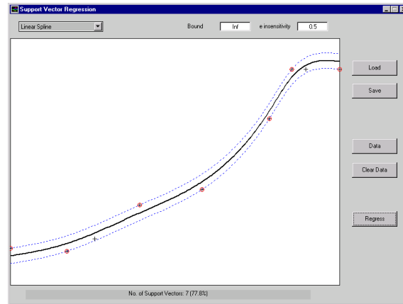
FIGURE 5.5: Spline Regression
